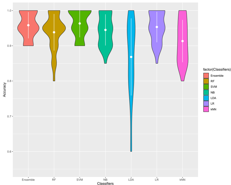
Figure 19: Accuracies Comparison
