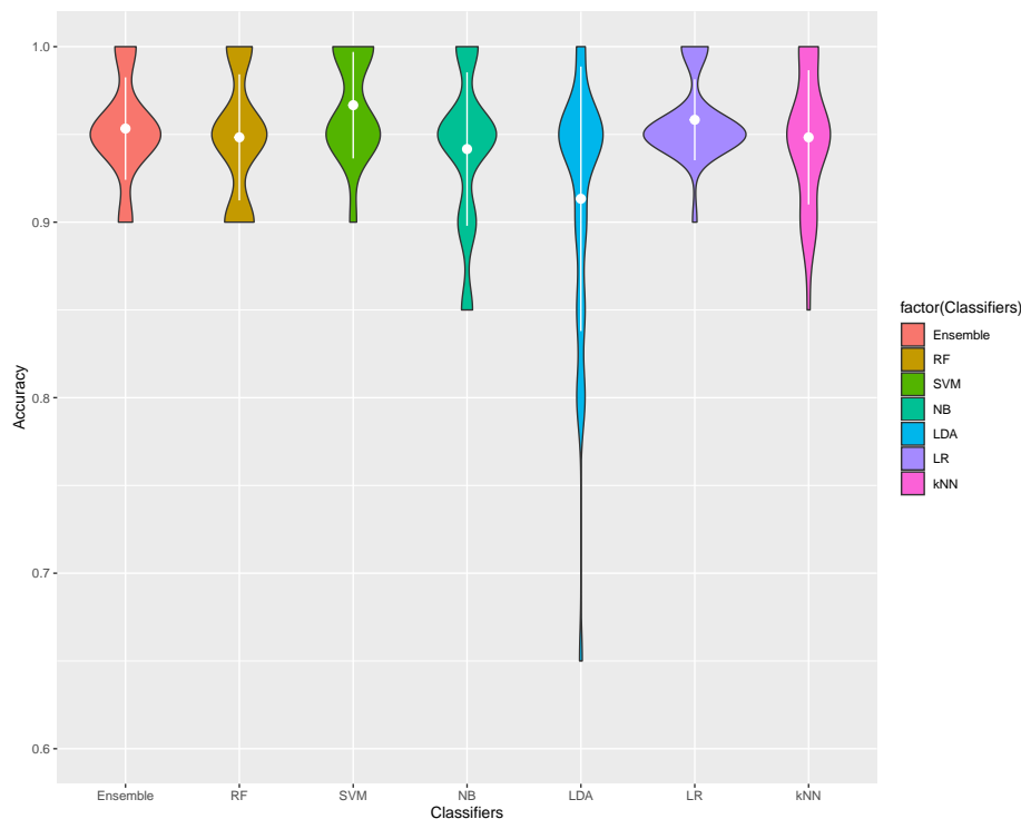
Figure 15: Accuracies Comparison The violin plot highlights the classification accuracy of each classifier, computed at each iteration; a black dot represents a specific accuracy value while the shape of each “violin” is drawn by a Gaussian kernel density estimation. Averaged accuracies and standard deviations are represented by white dots and lines.
