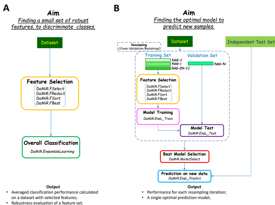
Figure 11: The DaMiRseq machine learning workflows
