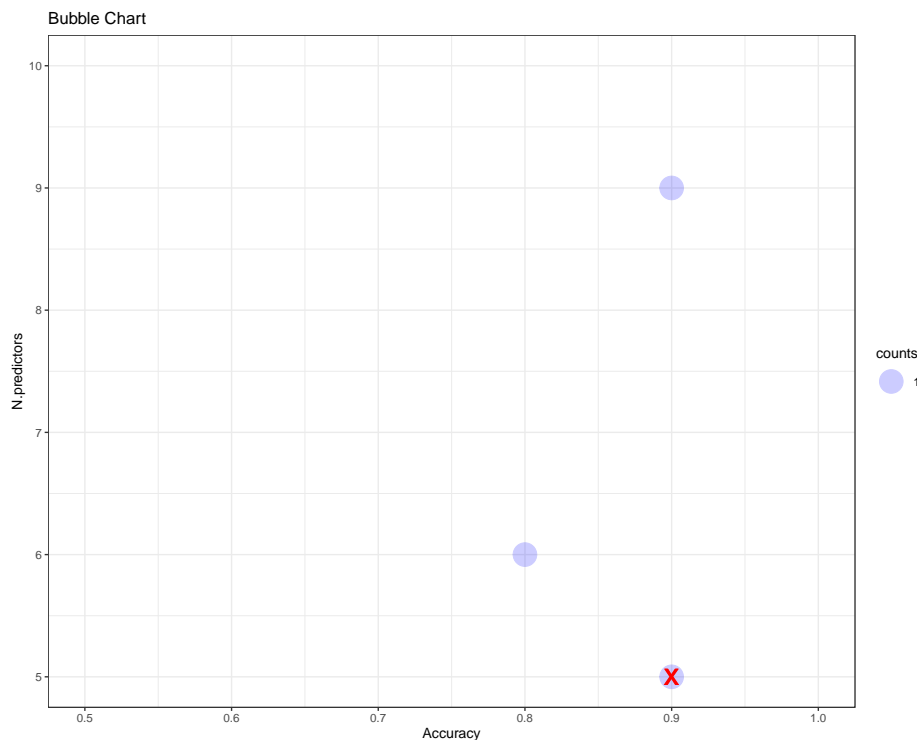
Figure 16: Bubble Chart
