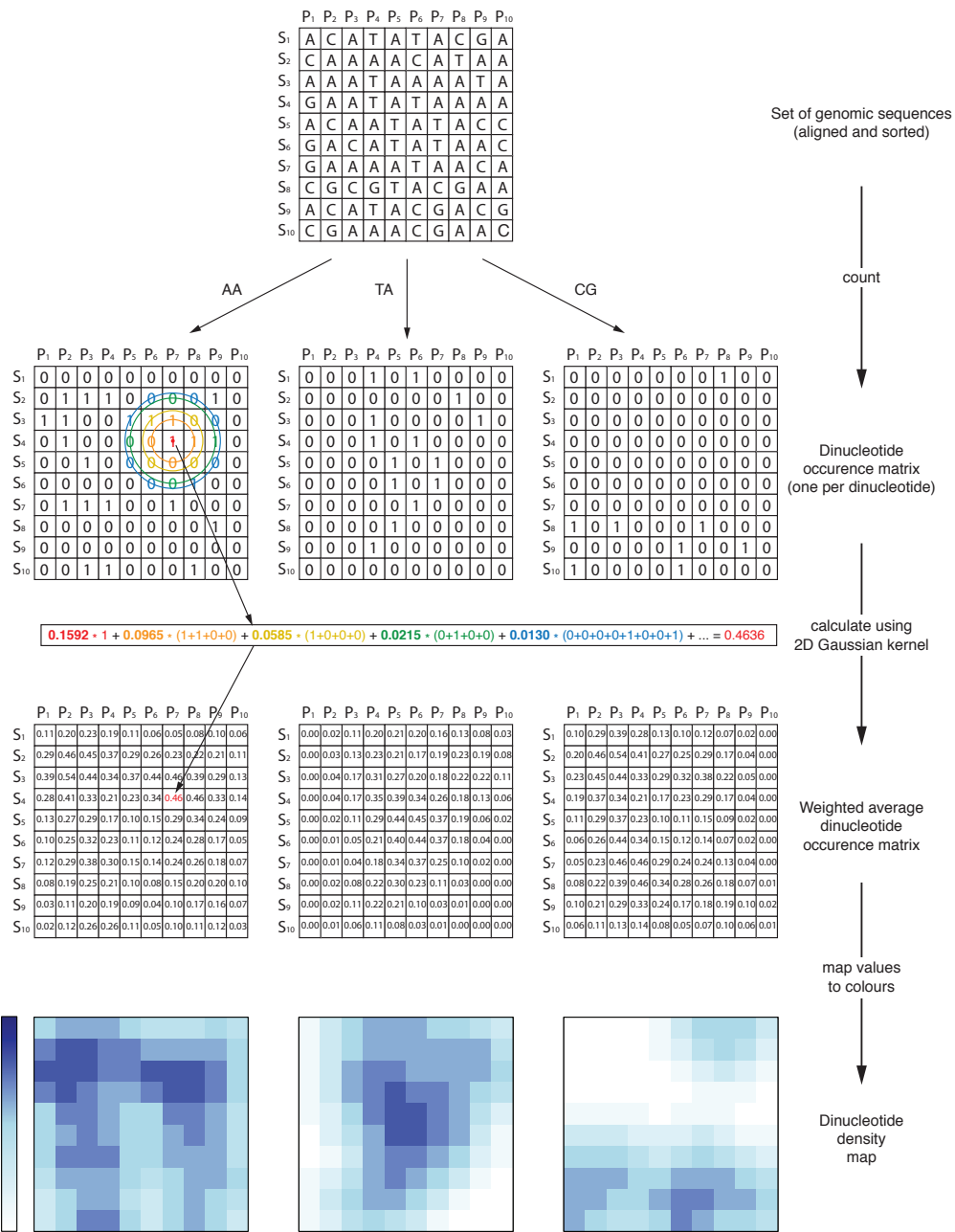
Figure 3: Schematics illustrating steps in pattern density calculation and visualisation. Genomic sequences (of the same length) are sorted and aligned into a matrix-like representation. Marking the presence of selected dinucleotide by 1 and the absence by 0 creates an occurrence matrix. Next, a weighted average is calculated at each position by placing a 2D Gaussian kernel at that position and assigning weights to surrounding positions. An example of calculating the value at position S 4 ,P 7 is shown. Surrounding positions are coloured on the basis of the weights assigned to them by the Gaussian kernel (bandwidth=5 in both dimensions, and covariance=0 between the two dimensions). Averaged values are mapped to different shades of blue to visualise the dinucleotide density.
