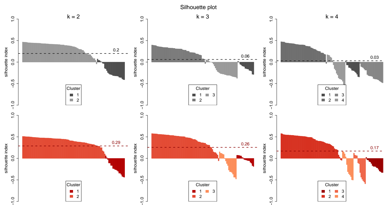
Figure 6: Silhouette graph for the classification of scaled peaks. In the top panel, Silhouette plots for the classification without alignment, as function of the number of clusters; in the bottom panel, Silhouette plots for the classification with alignment.
