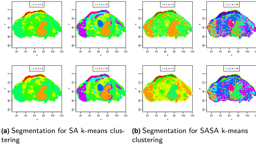
Figure 4: The spatial segmentations for spatially-aware (SA) and spatially-aware structurally-adaptive (SASA) k-means clustering with varying smoothing radii ( r = 1, 2 ) and number of segments ( k = 5, 10 )
